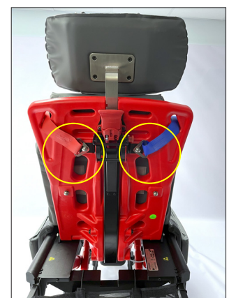
Cross-Strap harness attachment at back of backrest
