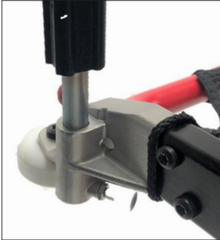
Insert push pole until it locks into place
